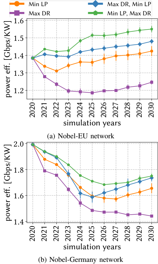
Fig. 5: Comparison of power-efficiency.
