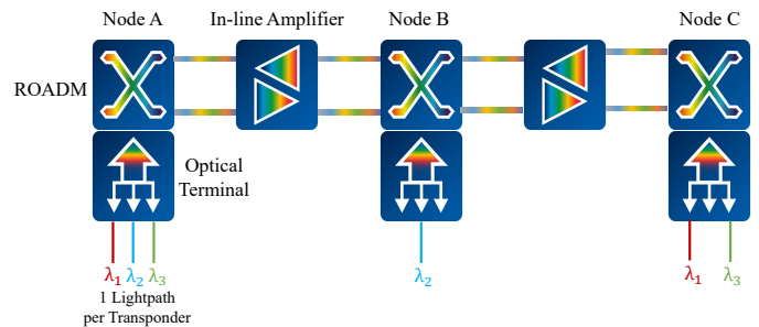
Fig. 1: Architecture of a long-haul optical transmission. Each optical terminal contains multiple software tunable BVTs. Every BVT is configured with one lightpath.
