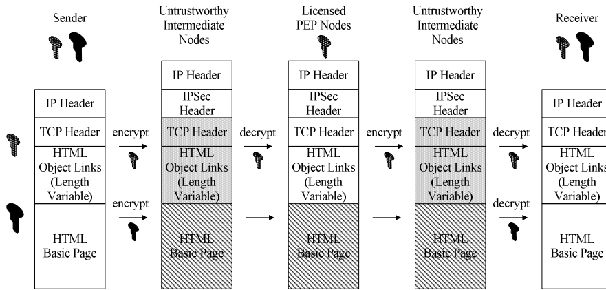
Fig. 1. CZML-IPSec transport mode protection model for TCP/HTTP
