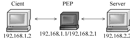
Fig. 3. CZML-IPSec transport mode testbed
