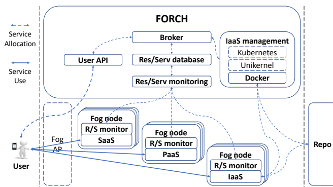
Fig. 1. FORCH reference architecture.
