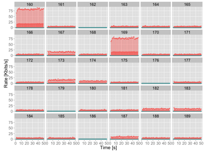
(b) erase message processing overhead in the DFN topology with 160 consumers.
