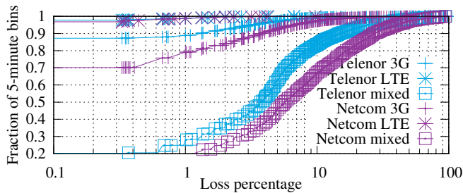
Fig. 5: Loss rate for 3G, LTE and when a RAT change is involved (mixed). Most loss happens in mixed category, LTE performs the best.
