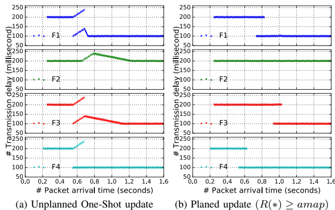
Fig. 7: Transient congestion during unplanned updates.
