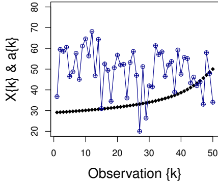
Figure 3: The decision values \{a_k\}_{k=1}^{50} (black points) and simulated server delay or load X_k (blue points) vs. observations k for horizon n = 50 ; the optimal data offloading time when k = 27, 29, 46, 47, 48 and 50 where X < a .
