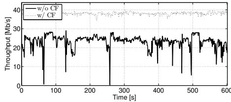
Fig. 4: Instantaneous aggregated client throughput before ( w/o CF ) and after ( w/ CF ) channel assignment.
