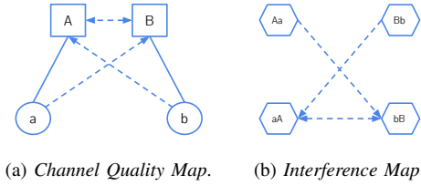
Fig. 3: Interference-Aware Channel Assignment. WTPs are represented as squares while LVAPs are represented as circles.
