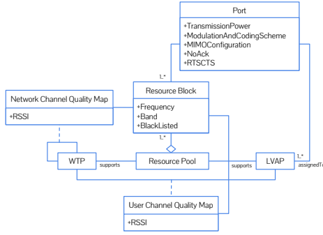
Fig. 2: The abstractions class-diagram.
