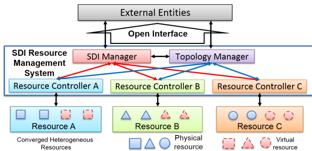
Fig. 2. High-level architecture of SDI resource management system
