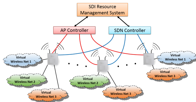
Fig. 3. High-level architecture for wireless access integration w/ SDI
