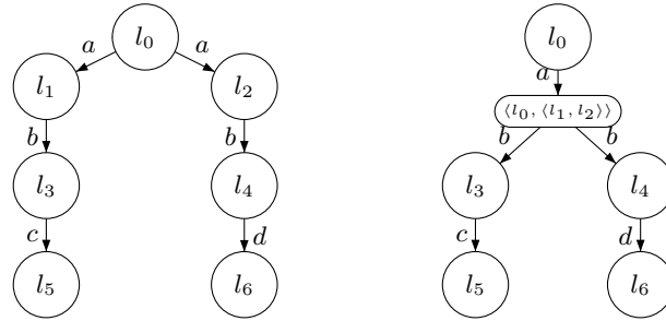
Fig. 3. Inherited nondeterminism may not decrease global lookahead.
