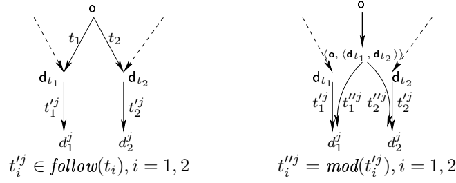
Fig. 2. Determinising 2 transitions: (left) before (right) after.
