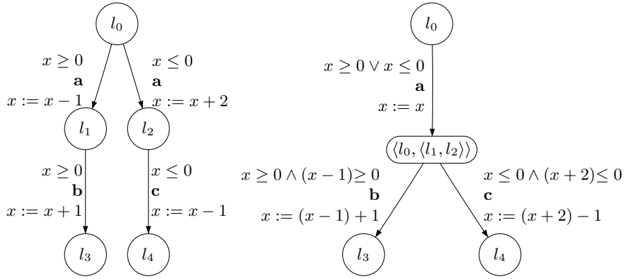
Fig. 1. Left: extended automaton \mathcal{S} Right: extended automaton \det(\mathcal{S})
