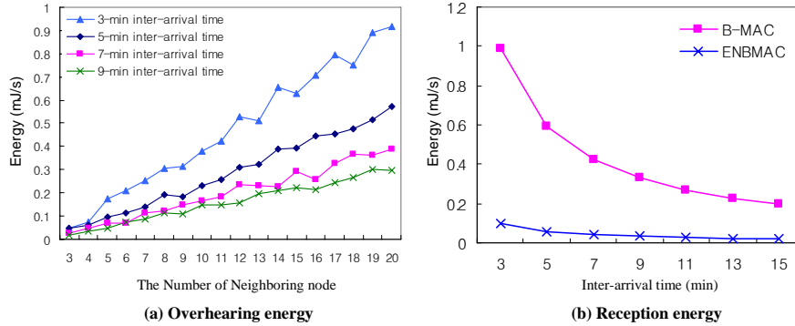
Figure 7. The result of multi-hop network
