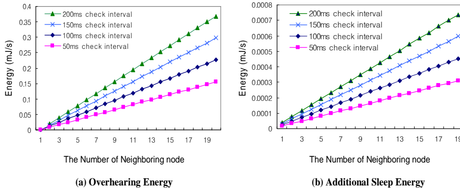
Figure 6. The result of simple network
