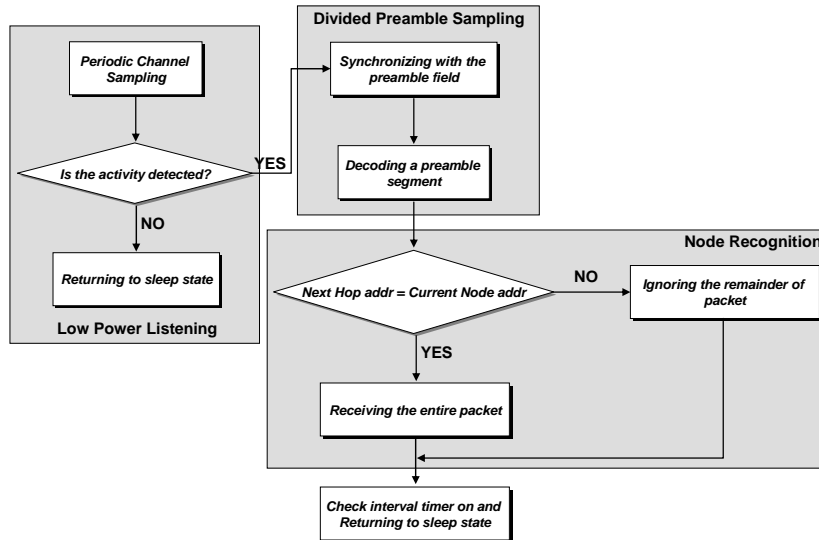
Figure 3. ENBMAC Subroutine - Reception
