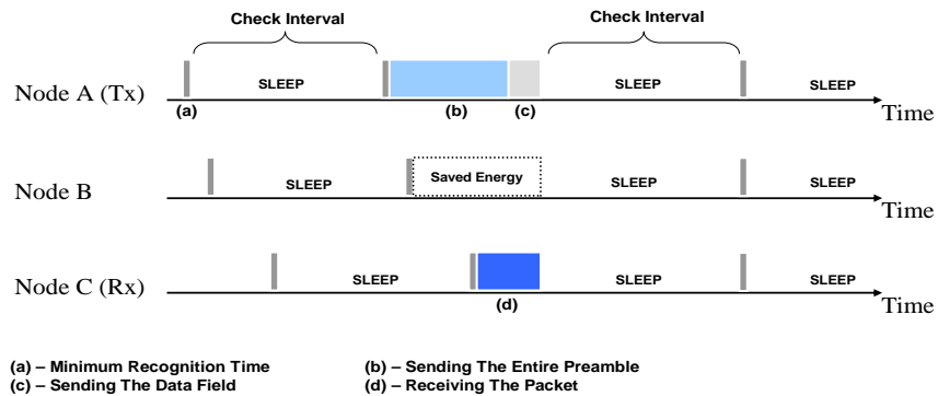
Figure 5. The basic operations of ENBMAC protocol
