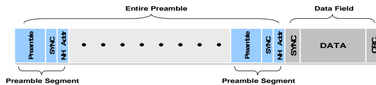
Figure 4. The Structure of ENBMAC Frame
