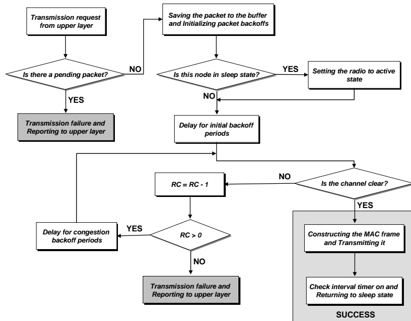
Figure 2. ENBMAC Subroutine - Transmission
