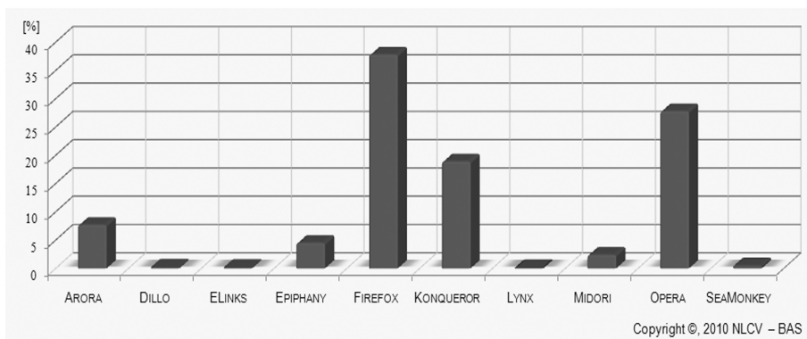
Fig. 5. Percent distribution of accomplished attacks to Linux OS with respect to the separate Browser Systems
