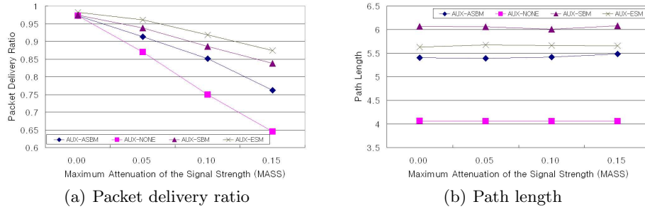
Fig. 5. Performance comparison of AUX routing using various link stability models.
