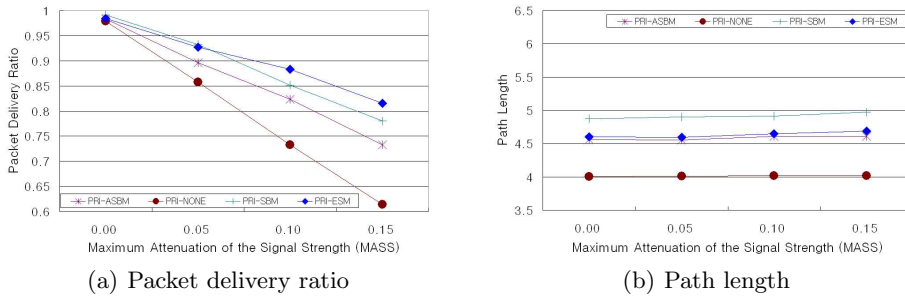
Fig. 4. Performance comparison of PRI routing using various link stability models.
