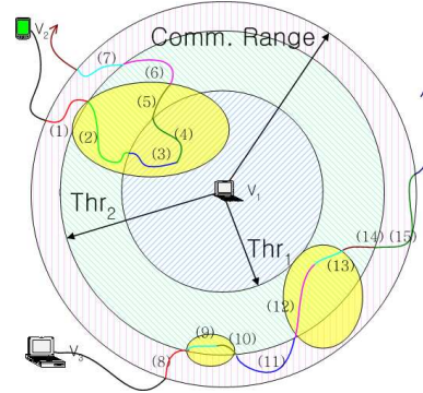
(b) Estimation results
