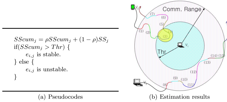
Fig. 1. Pseudocodes and estimation results of SBM.
