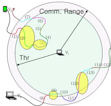
(b) Estimation results
