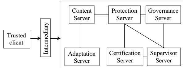
Fig. 1. DMAG-MIPAMS architecture
