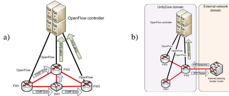
Fig. 6. ICMP topology discovery (a) and ARP search (b).
