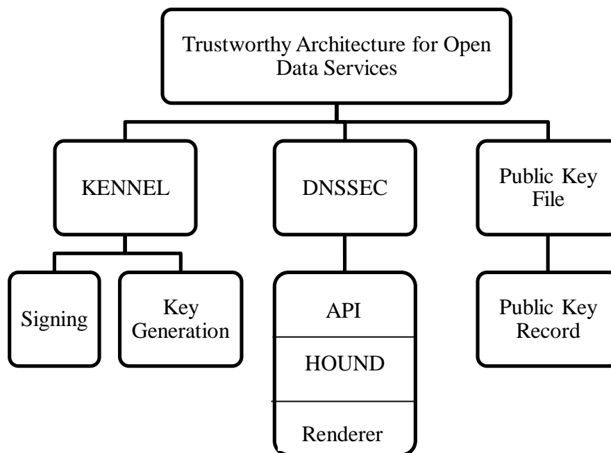
Fig. 1. Trustworthy Architecture for Open Data Systems
