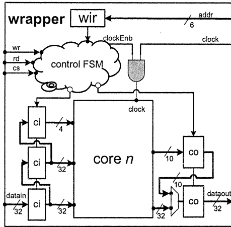
Figure 3. Wrapper scheme.
