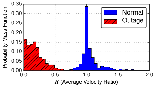
Fig. 3: Distribution of Average Velocity Ratio for normal and outage durations.
