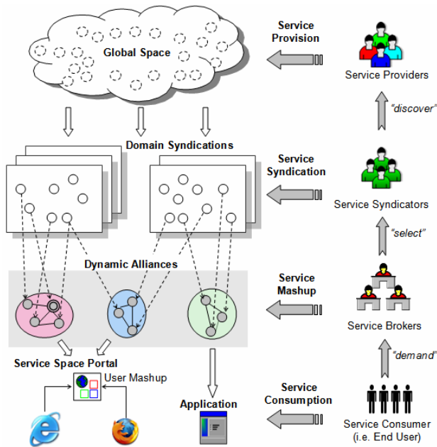
Fig. 8. Proposed Architecture
