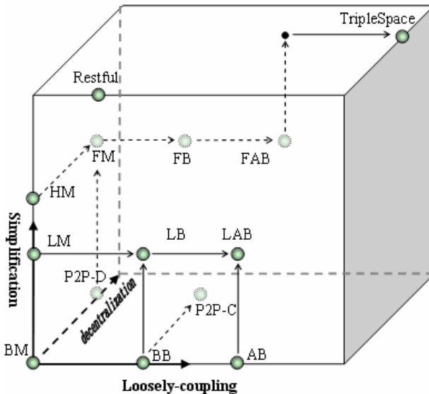
Fig. 7. Evolutionary Cube
