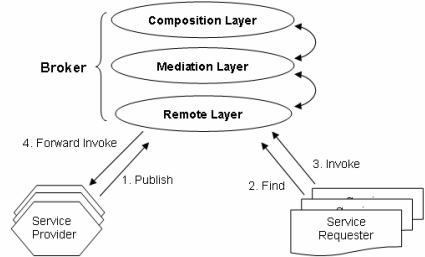
Fig. 2. Layered Broker Style
