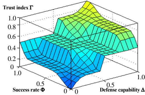
Fig. 3. Variation of trust index \Gamma with respect to the variations of job success rate \Phi and intrusion defense capability \Delta at each resource site
