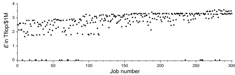
Fig. 8. Improved Grid performance/cost ratio for 300 jobs allocated to 6 resource sites after trust integration and security upgrade
