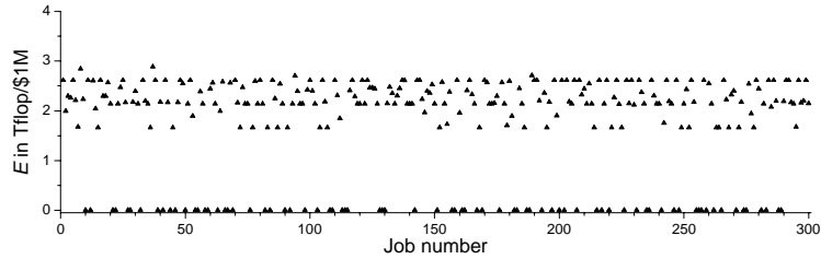
Fig. 7. Grid performance/cost ratio for 300 jobs allocated to six resource sites with fixed trust index and no site security reinforcement
