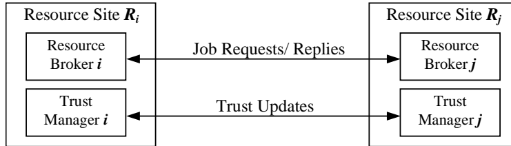
Fig. 1. Securing Grid resources with trust integration and resource brokerage
