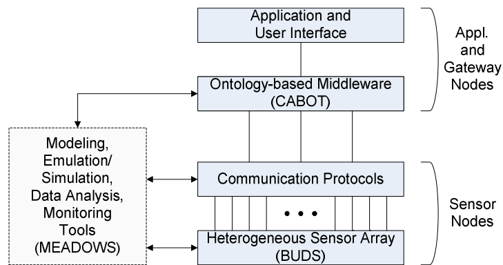
Figure 1: The BLOSSOMS system architecture.
