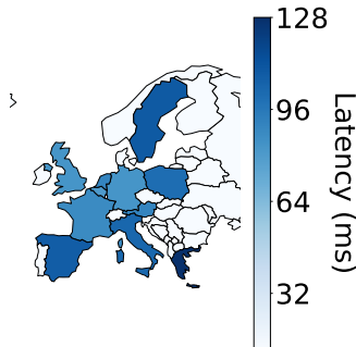
Fig. 4: Heatmap of median latencies in 2024 in Europe from the Cloudflare Radar.
