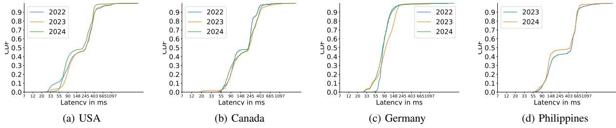
Fig. 3: CDF of RIPE Atlas TLS latencies in the USA, Canada, Germany, and the Philippines from 2022 to 2024.
