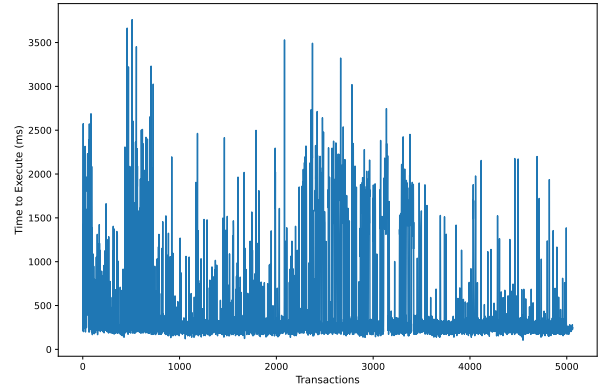
Fig. 6. Time needed for all the transactions by the water supplier for a 24-hour billing period and 82 clients.
