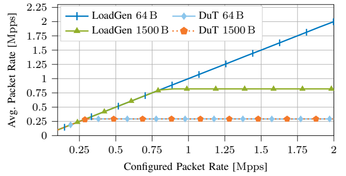
Fig. 5. Throughput of the Linux router
