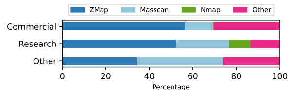
Fig. 3: Scanning tools spread per category of organization.
