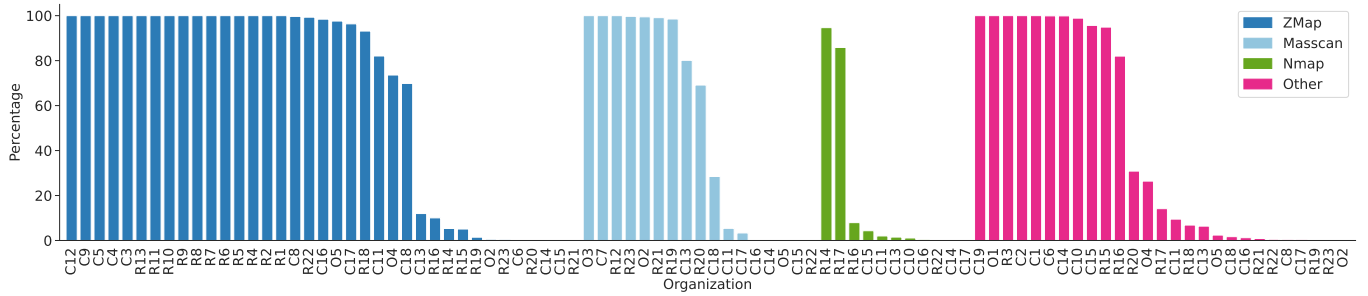
Fig. 2: Percentage of packets sent with the respective scanning tool for each identified organization. Labels as defined in Fig. 1.
