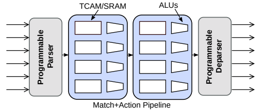
Fig. 1: PISA Architecture.
