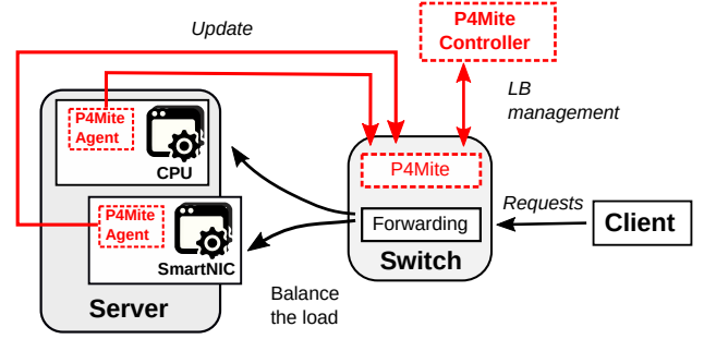
Fig. 2: P4Mite overview.
