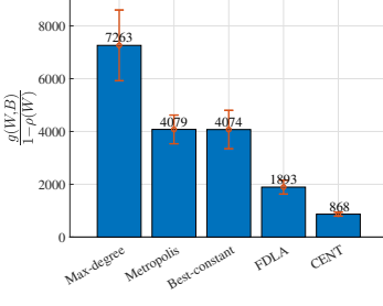
Fig. 5. Training time objective \frac{g(W,B)}{1-\rho(W)} .
