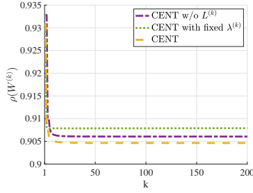
Fig. 2. Convergence factor \rho(W) vs. steps.
