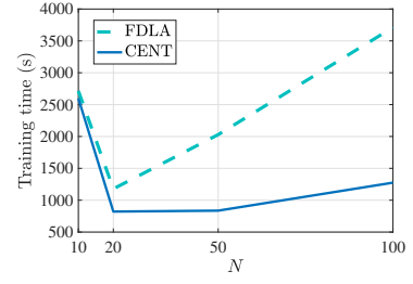
Fig. 7. Wall-clock training time over N .
