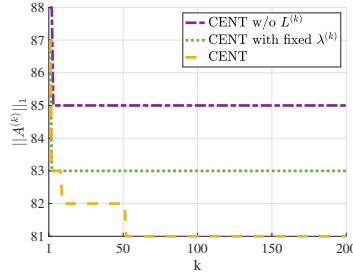
Fig. 3. Number of selected links vs. steps.
