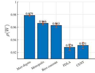
Fig. 4. Convergence factor \rho(W) .
