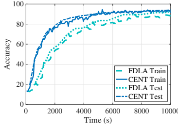
Fig. 6. Accuracy vs. wall-clock time.
