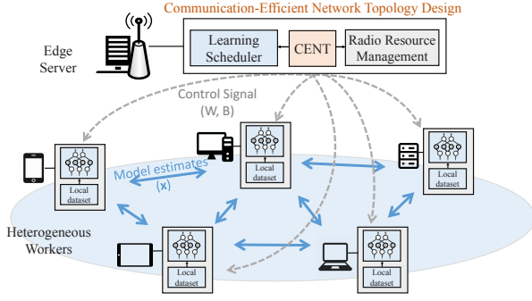
Fig. 1. CENT for decentralized ML.
