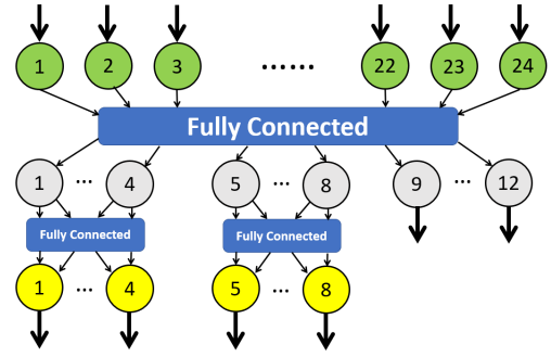
Fig. 9: Example of a 3-stage Clos structure from [16]
