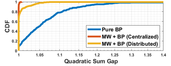
Fig. 10: Quadratic Sum Gap Comparison (Clos)
