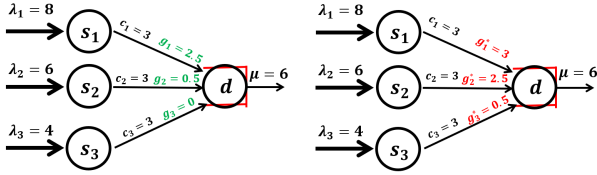
Fig. 5: Example that (9) does not achieve most balanced overload with limited capacity with \gamma \rightarrow \infty , where node d has bounded buffer. On the left, (g_1, g_2, g_3) = (2.5, 0.5, 0) denotes the transmission rates under (9) in steady state, under which \dot{\mathbf{q}} = [5.5, 5.5, 4] . It is not the most balanced overload as presented on the right, where \dot{\mathbf{q}}^* = [5, 3.5, 3.5] under (g_1^*, g_2^*, g_3^*) = (3, 2.5, 0.5) , the optimal solution to (3). Other \gamma values also suffer from the suboptimality.
