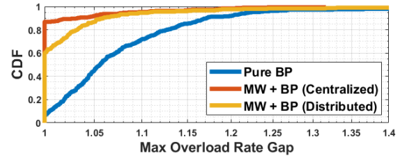
Fig. 11: Max Overload Rate Gap Comparison (Clos)
