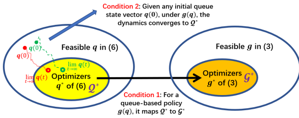
Fig. 4: Condition 1 (existence) and 2 (convergence) to verify that a queue-based policy achieves most balanced overload
