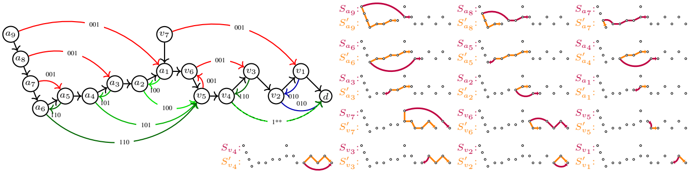
Fig. 2. Topology where multiple TAG values should be matched by wildcard rule w for out-link p_{v_4} . Black links are t_s links on the SPT and have unit cost. p_s links are colored according to their TAG values. The ones reverse to the SPT have unit cost, the other p_s links have cost one plus their SPT distance, e.g., c(v_7, v_1) = 8 , except c(v_4, d) = 6 , c(a_6, v_5) = 10 , and c(a_4, v_5) = 7 . In the small figures the SPDP-segments S_v and S'_v from each node are drawn with purple and orange, respectively.
