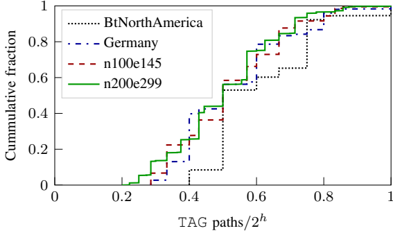
(b) Cumulative distribution function of tag space density. |P|/2^h = 0.5 means that s finds a new path for every second try on average.
