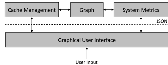
Fig. 1. CacheMAST architecture.
