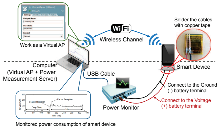
Fig. 1. Experiment setup for studying the relations between network metrics and power consumption
