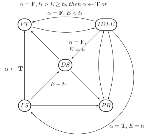
Fig. 8. Power state transition model
