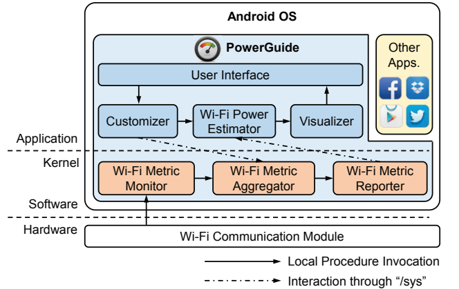
Fig. 9. Implementation Architecture of PowerGuide
