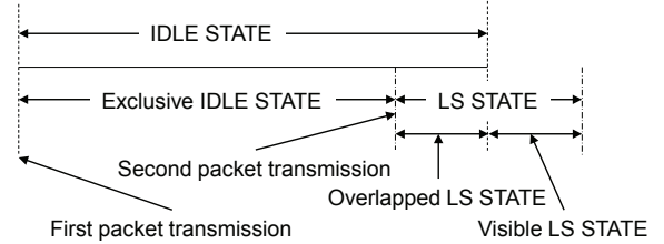
Fig. 5. IDLE and LS state illustration
