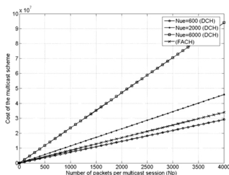
Fig. 5. Cost of the multicast scheme against N_p for different transport channels
