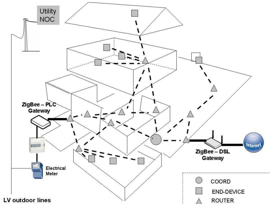
Figure 9: ZB Smart-House - Positions of the devices
