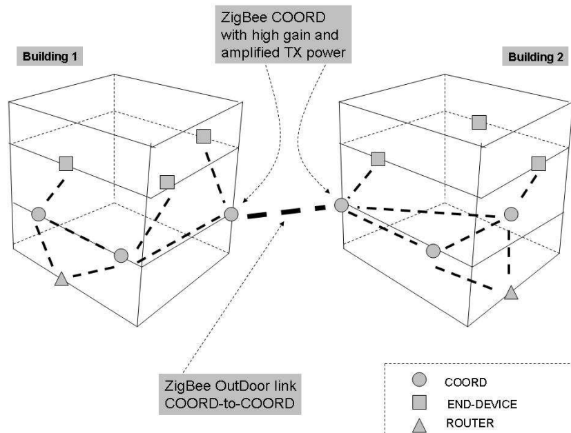
Figure 6: OutDoor two-buildings ZigBee applications
