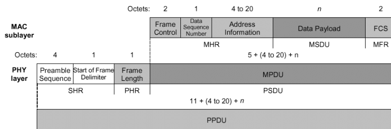
Figure 7 : Data frame format in IEEE 802.15.4
