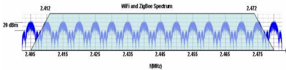
Figure 3: Wi-Fi and ZigBee spectrum
