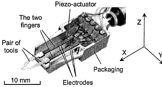
Figure 1: Overview of the microgripper.
