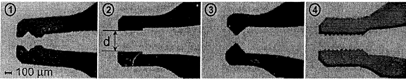
Figure 2: Different kinds of pair of available tools. These tools are made of Nickel, are 200\ \mu\text{m} thick and have been fabricated by UV LIGA. d is the initial gap between both tools.
