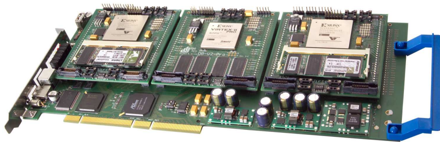
Fig. 5. RAPTOR2000/X64 rapid prototyping environment.
