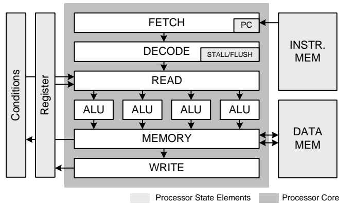
Fig. 7. VLIW architecture.
