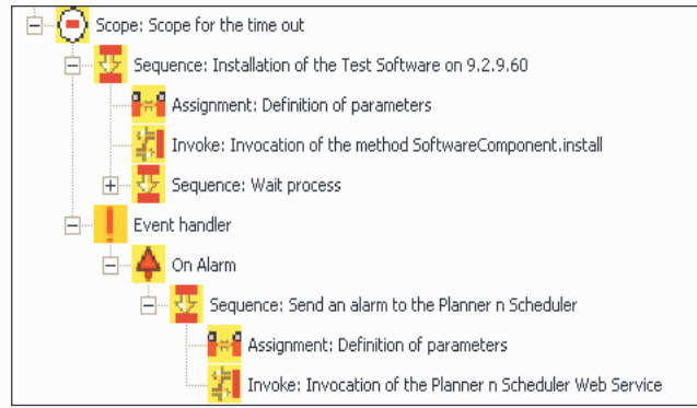
Fig. 8. Enforcing Deadlines and Durations
