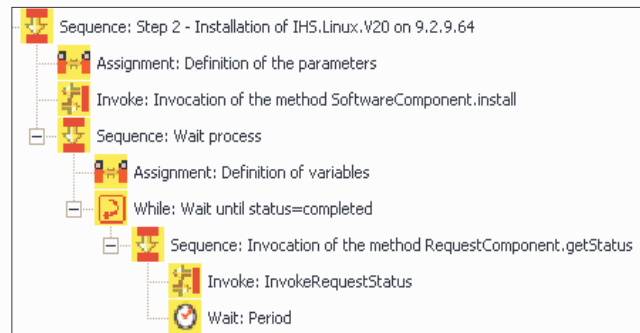
Fig. 7. Monitoring Task Execution Status
