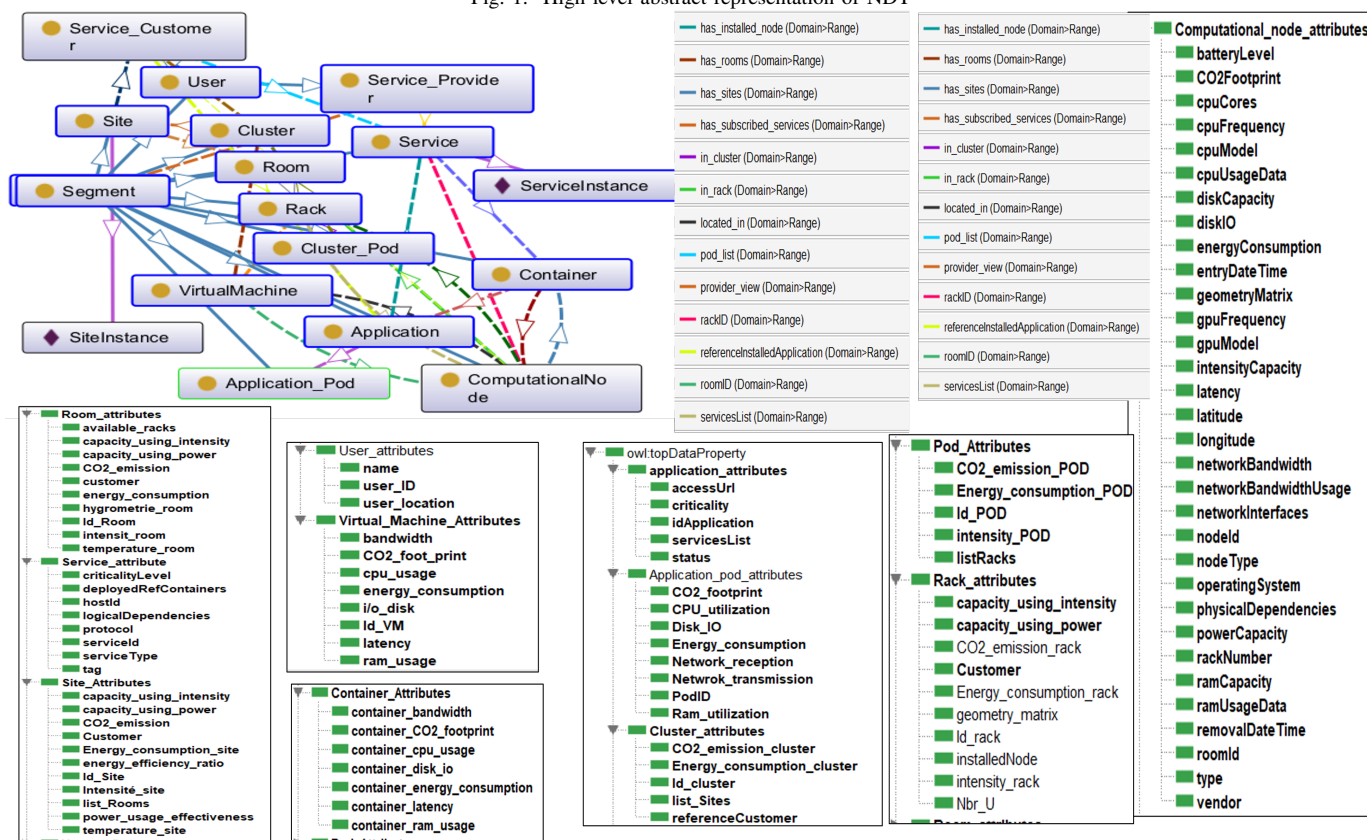
Fig. 2. Detailed Ontology representation
