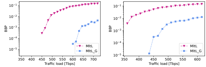
Fig. 7: BBP for request type YouTube . US26 topology (left) and Euro28 topology (right).
