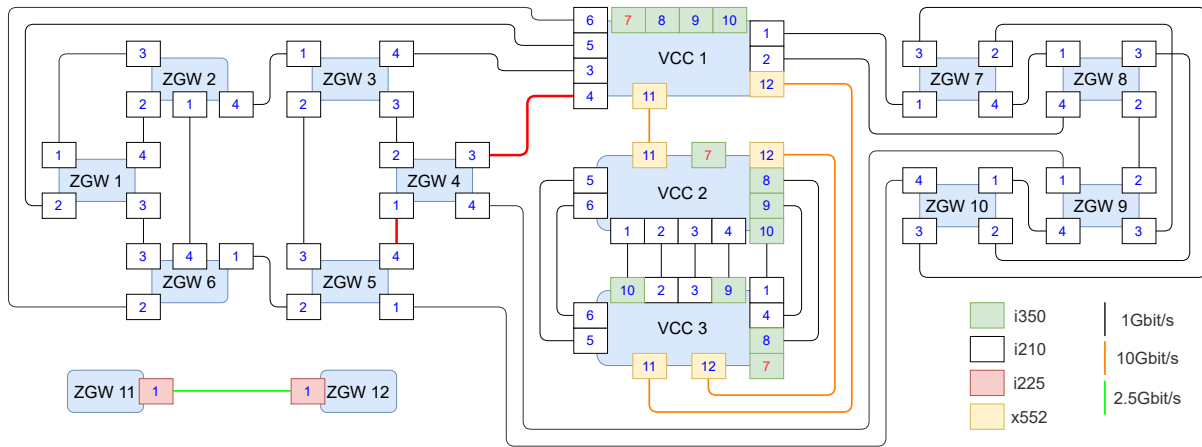
Figure 5: EnGINE network overview with connections for presented use-case marked in red
