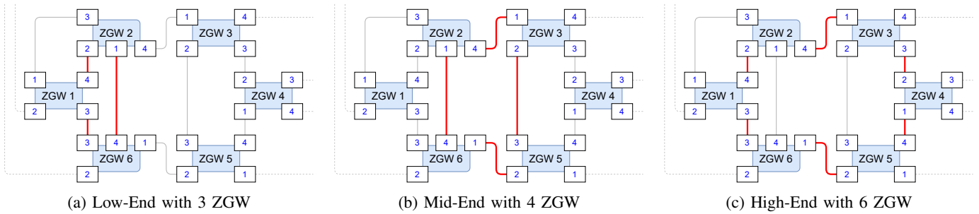
Figure 2: Sample configurations for various IVN complexities. Red lines show links used in the respective configurations.
