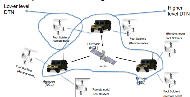
Figure 2: Network Model
