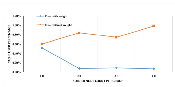
Figure 3: Cache Miss
