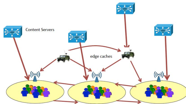
Figure 1: Content Caches
