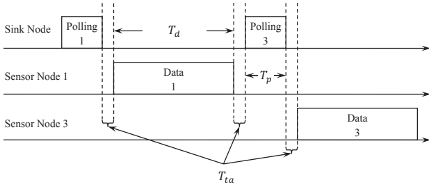
Fig. 1. Illustration of a polling-based WSN MAC protocol.
