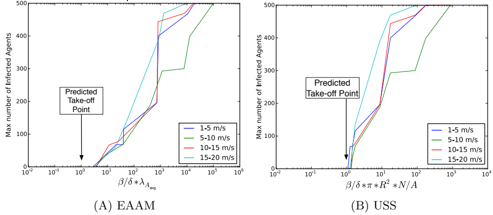
Fig. 4. Accuracy of Framework Approximations. Random Waypoint Take-off plots for EAAM and USS.
