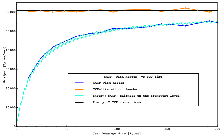
Fig. 4. Goodput, if the header is taken into account
