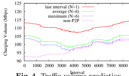
Fig. 4. Traffic volume prediction.
