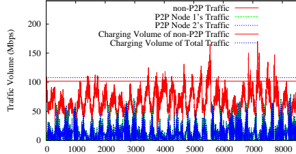
Fig. 6. P2P capacity utilization when using capacity sharing algorithm.
