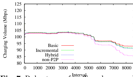
Fig. 7. Robustness of traffic volume prediction algorithms.
