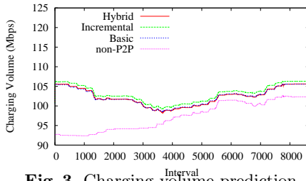
Fig. 3. Charging volume prediction.
