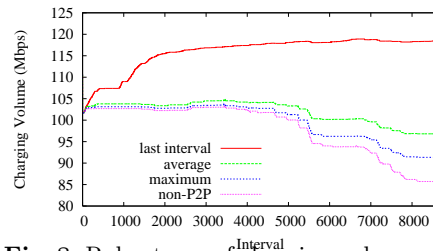
Fig. 8. Robustness of charging volume prediction algorithms.
