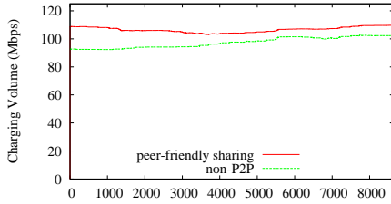
Fig. 5. Charging volume when using capacity sharing algorithm.
