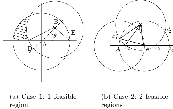
Fig. 2. Computation of the non-interfering zone (dashed)
