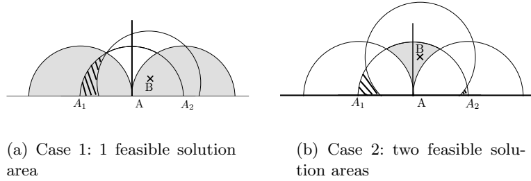
Fig. 1. Computation of P_{12}(k) (the non-interfering zones are dashed)
