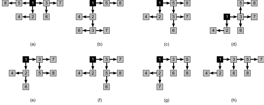
Fig. 2. All possible tree restructuring results for the case depicted in (e) of Fig. 1: (a) due to the Type-A transformation; (b) and (c) due to the Type-B transformation; (d) due to the Type-C transformation; (e) to (h) due to the Type-D transformation.
