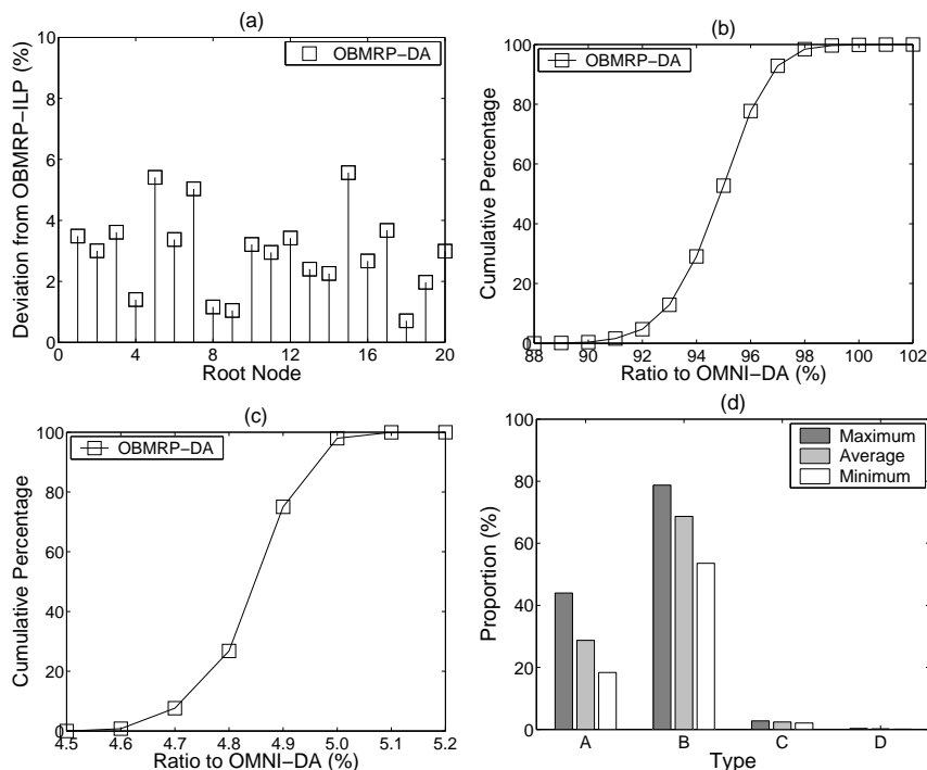
Fig. 3. Efficacy of OBMRP-DA: (a) \bar{L} performance compared with OBMRP-ILP; (b) \bar{L} performance compared with OMNI-DA; (c) Control overhead compared with OMNI-DA; (d) Distribution of transformation operations.
