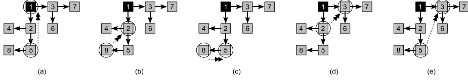
Fig. 1. Snapshot of the five distinct cases where a tree restructuring request from node i will be considered by node j . Both node i and node j are marked by circles. Node j is pointed by the double arrow.
