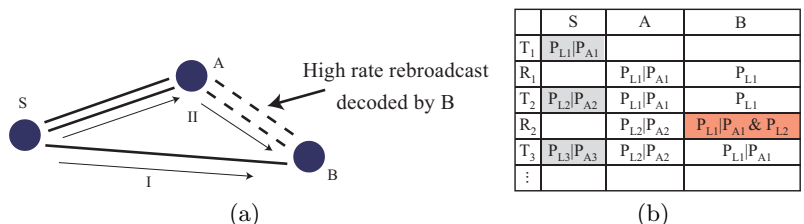
Fig. 2. (a) Two different rates of information available at node B: flow I, low rate information and flow II, high rate information. (b) Packet transmission and reception schedule.
