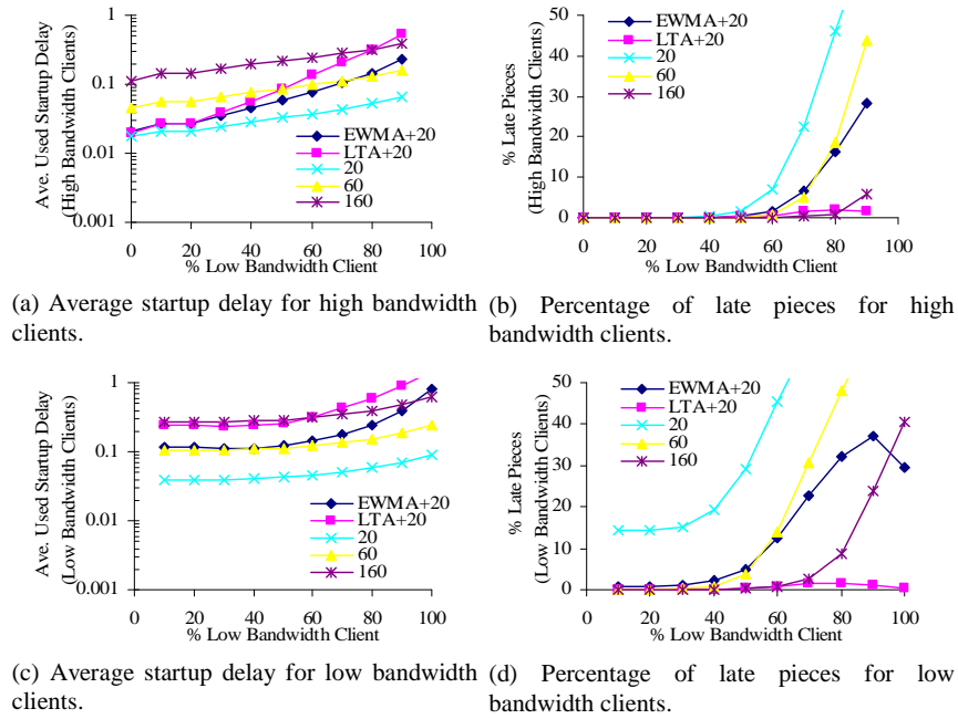
Fig. 11. Performance with heterogeneous clients ( \lambda = 64 , \phi = 0 , U_L = 0.4 , D_L = 1.2 , U_H = 2 , D_H = 6 ).
