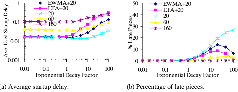
Fig. 10. Performance with an exponentially decaying arrival rate ( U=2 , D=6 , \lambda(t) = \lambda_0 e^{-\gamma t} , \lambda_0 = 128\gamma / (1 - e^{-2\gamma}) ).
