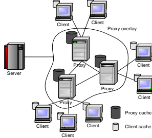
Fig. 1. The COPACC architecture.
