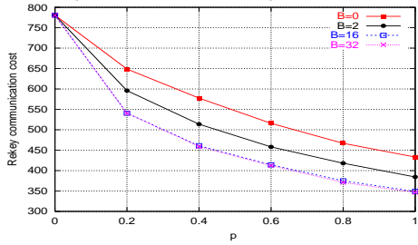
(g) Probabilistic shifting on LOG_m
