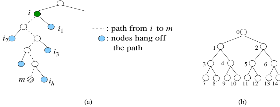
Figure 2: Static SDR key tree
